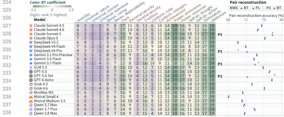
Figure 5: Value orientations of the 22 models. Left: centered BT coefficients (color) and ranks (digits), grouped by higher-order value group. Right: in-sample accuracy of BT and Plackett-Luce (PL) in reproducing pairwise comparisons. Squares show BT fitted to P3 choices.
