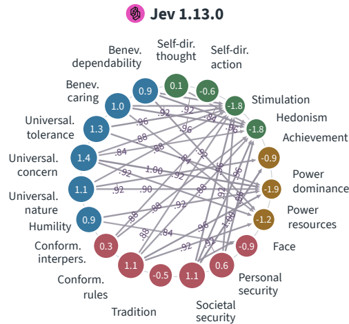
Figure 13: VALUEGRAPH of the Jev reference system. The panel shows the 30 edges with the largest |P| , estimated from Jev’s action scores (Table 7) and drawn on the scales of Figure 12.
