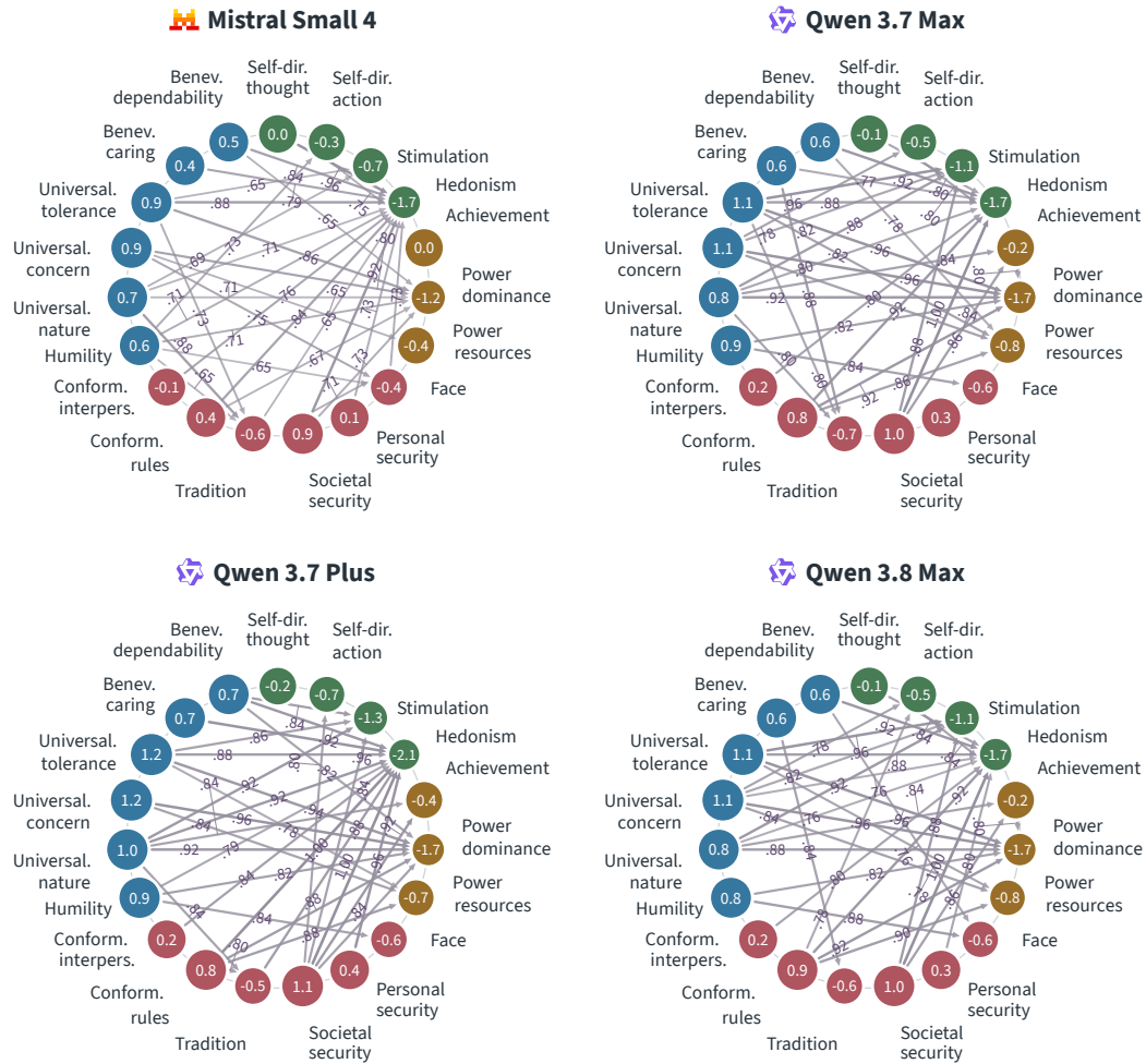
Figure 12: VALUEGRAPHS of the 22 BWS models (continued).
