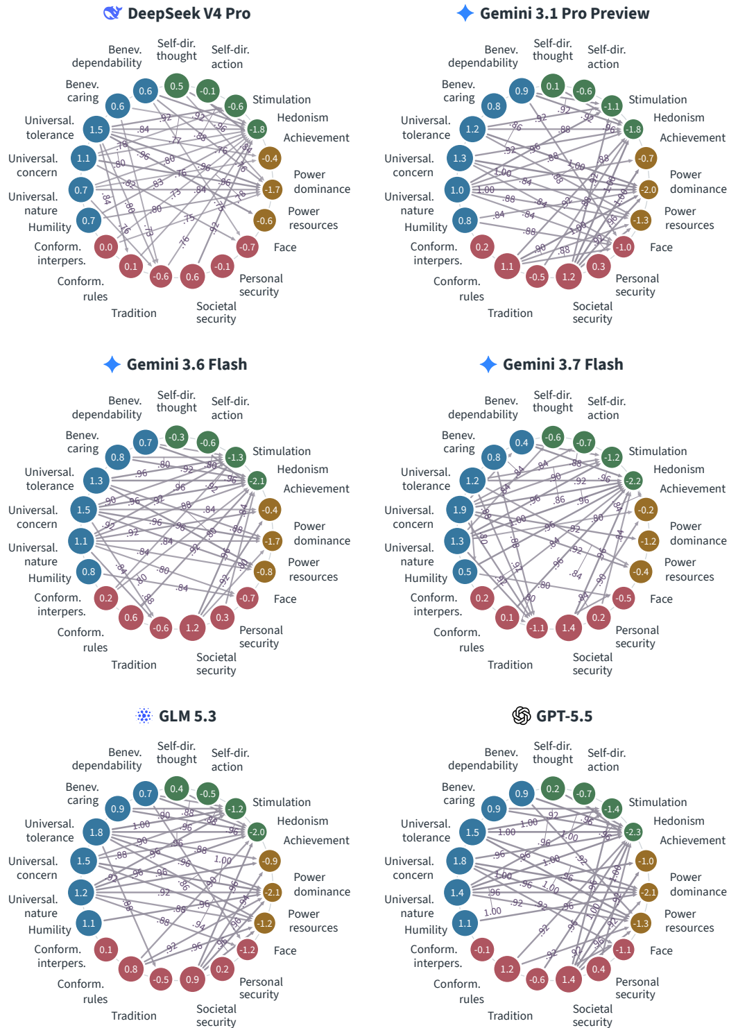
Figure 12: VALUEGRAPHS of the 22 BWS models (continued).
