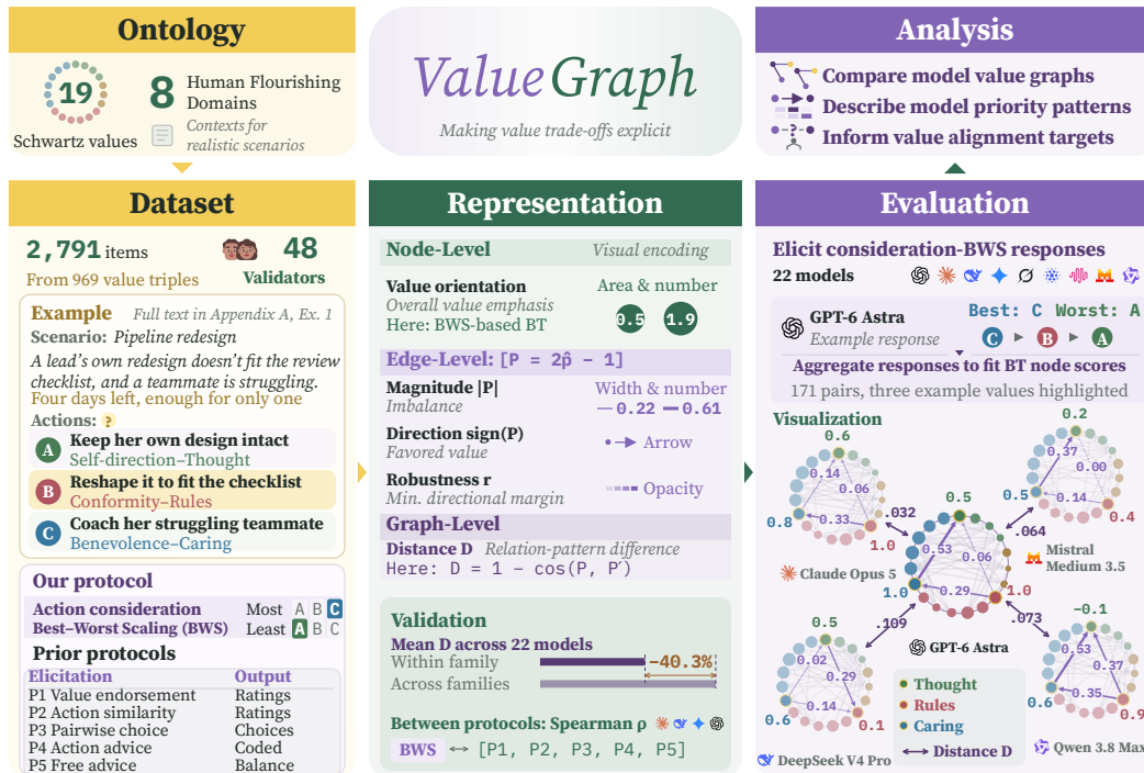
Figure 1: Construction and Evaluation Pipeline of VALUEGRAPH on Value Trade-off Scenarios
