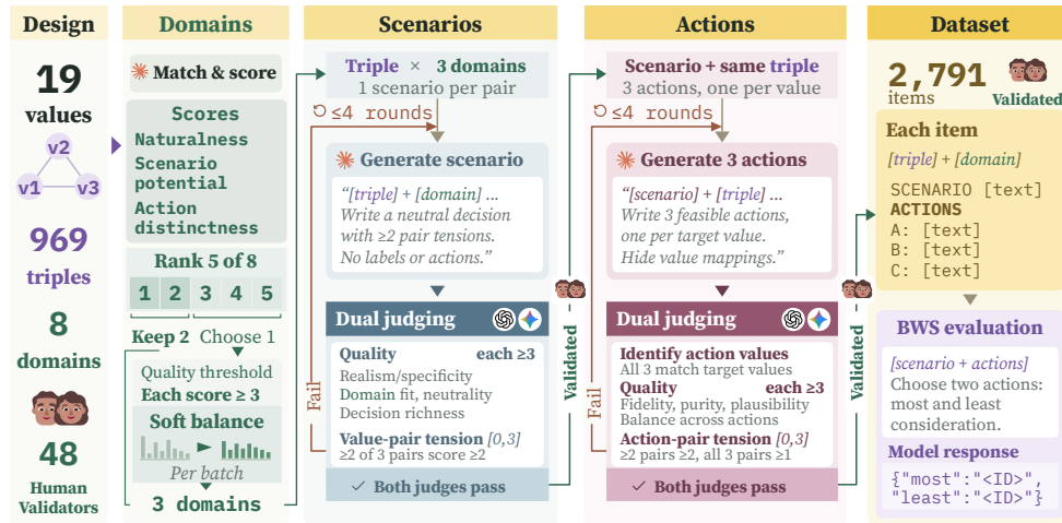
Figure 2: Dataset construction. Two independent judges assess each scenario and action set. A candidate passes only if both score every criterion at least 3 (1–5 scale) and the pair-tension thresholds hold, with up to four rounds. Stages marked Validated were also checked by 48 human validators.
