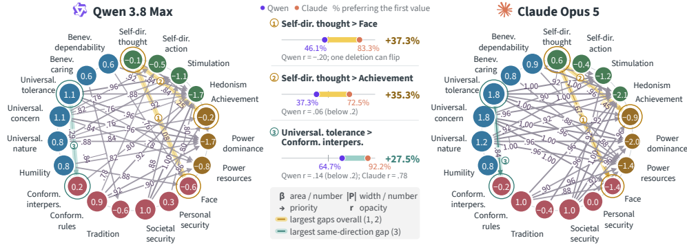
Figure 6: Edge-level comparison of Qwen 3.8 Max and Claude Opus 5. Gold halos mark the two largest probability gaps among all 171 pairs (1, 2), and the teal halo the largest among same-direction pairs (3). The middle panel lists both probabilities and their difference. Nodes show BT scores, edge labels |P| , and opacity r .
